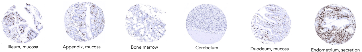
Images of normal tissue gallery of CD7 MSVA-007R
